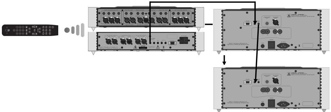
Figure 3: Remote Operation
