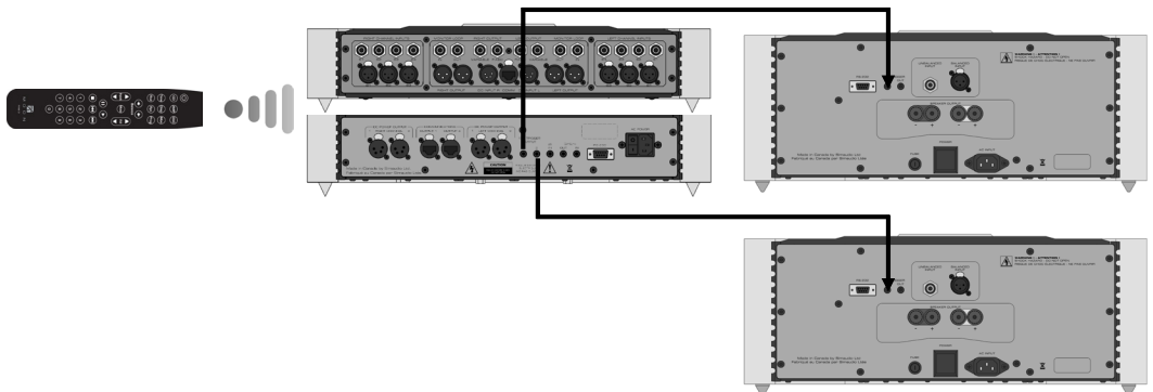
Figure 4: Remote Operation
