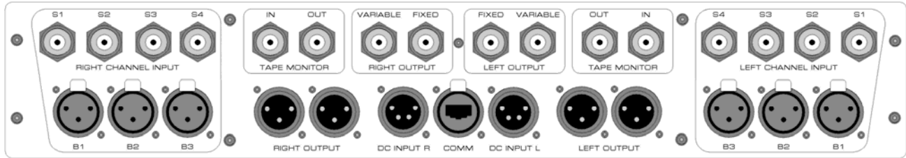
Figure 3: Rear panel of MOON P-8 Preamplifier
