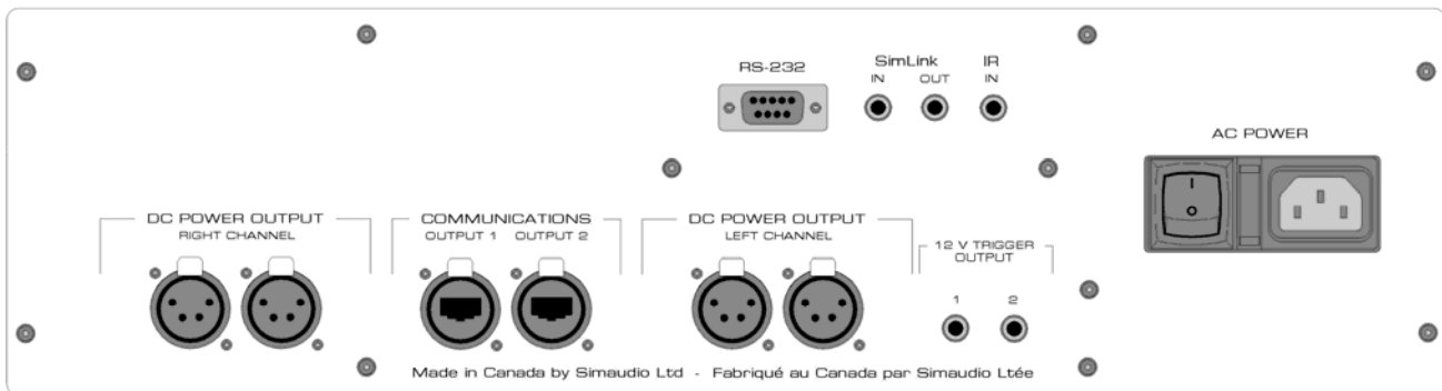
Figure 4: Rear panel of MOON P-8 Controller
