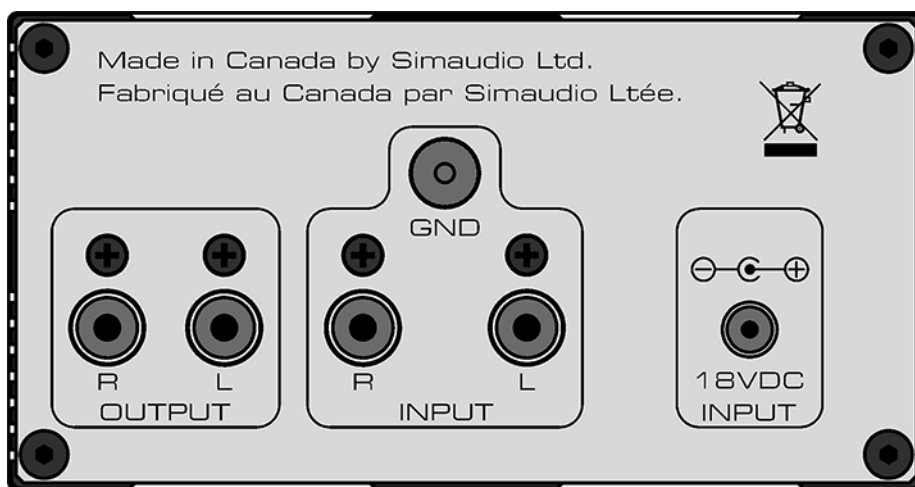
Figure 2: Rear panel of MOON 110LP
