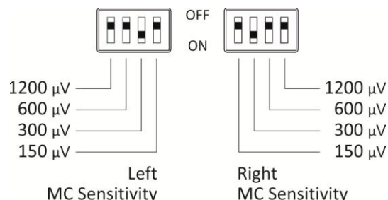
Fig.: Factory setting for sensitivity
