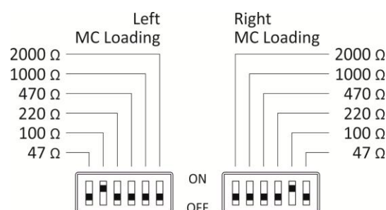
Fig. 2: Factory setting of terminating resistor
