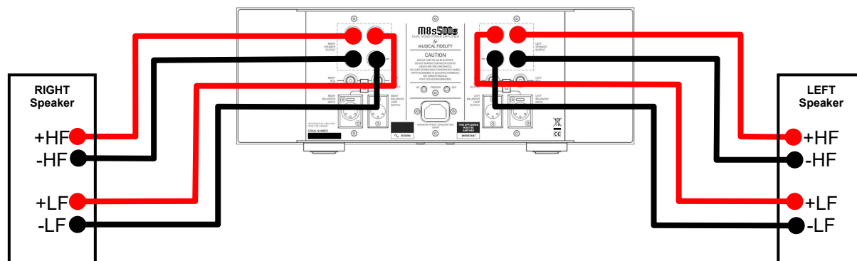
Rear view bi-wiring speaker leads connection diagram. (Preamp, trigger and mains leads omitted for clarity).
