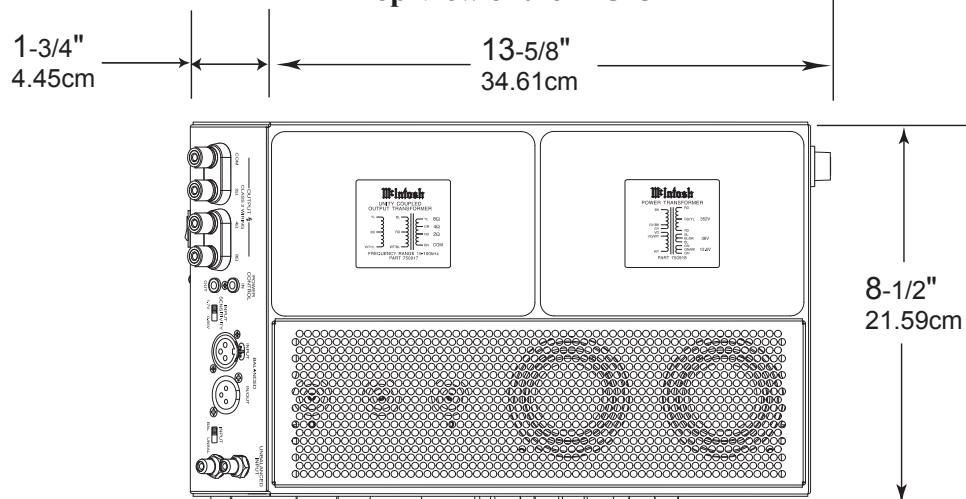
Top View of the MC75
