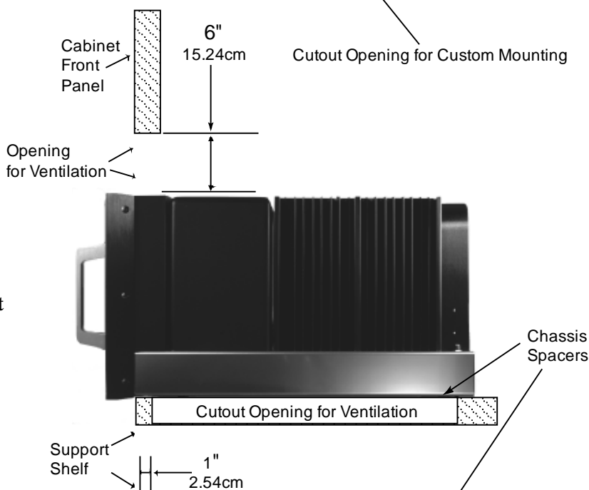
MC602 Side View in Custom Cabinet
