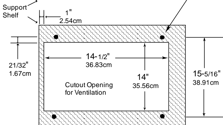
MC602 Bottom View in Custom Cabinet
