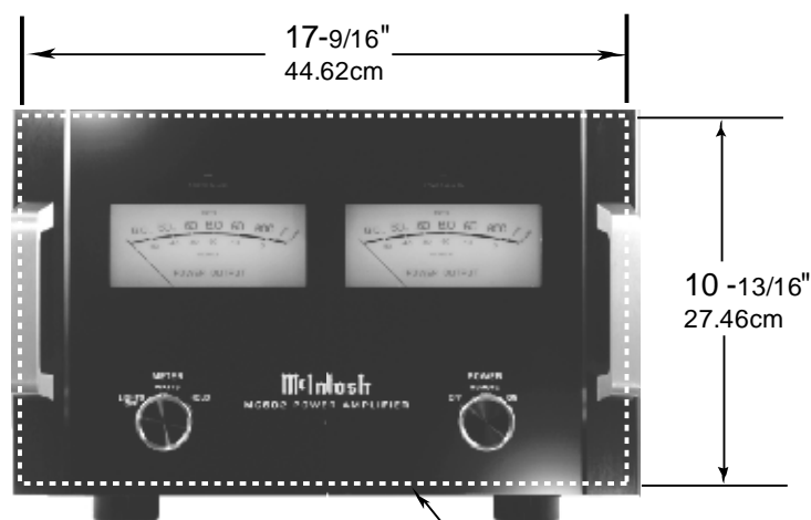
MC602 Front Panel Custom Cabinet Cutout
