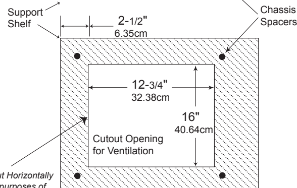
MC452 Bottom View in Custom Cabinet
