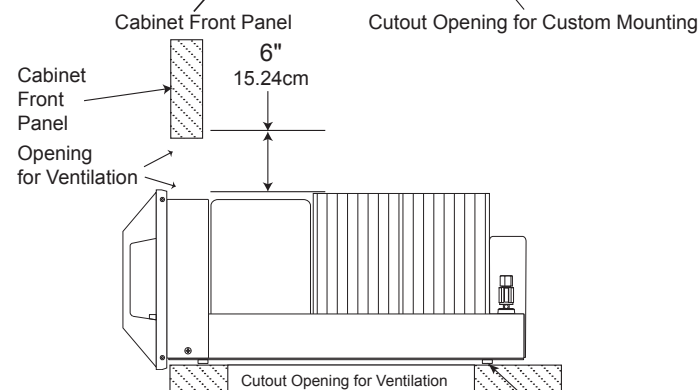
MC452 Side View in Custom Cabinet
