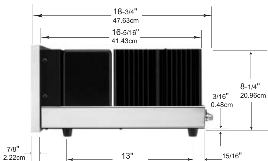
Side View of the MC402
