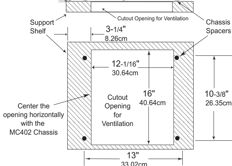
MC402 Bottom View in Custom Cabinet
