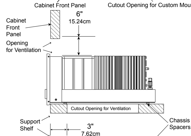
MC312 Side View in Custom Cabinet
