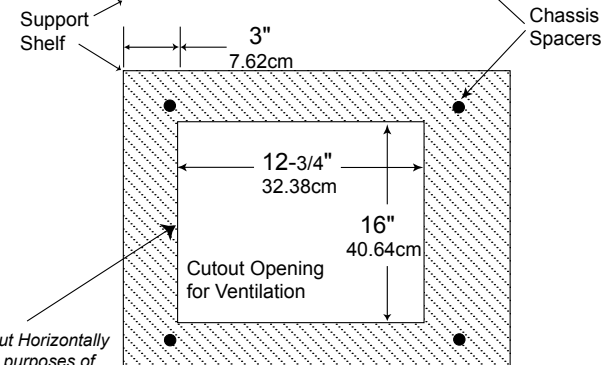
MC312 Bottom View in Custom Cabinet
