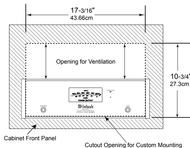
MC301 Front Panel Custom Cabinet Cutout
