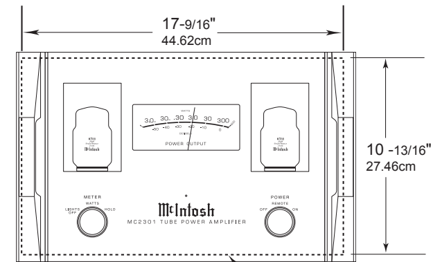
MC2301 Front Panel Custom Cabinet Cutout
