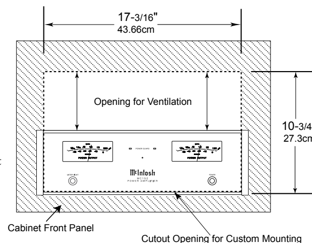
MC152 Front Panel Custom Cabinet Cutout
