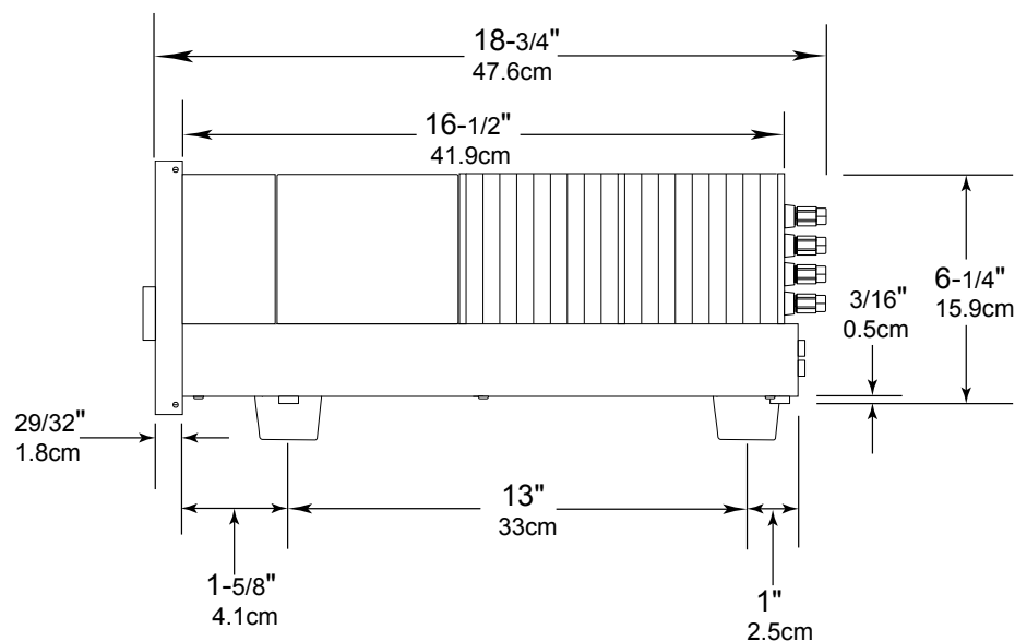
Side View of the MA7900
