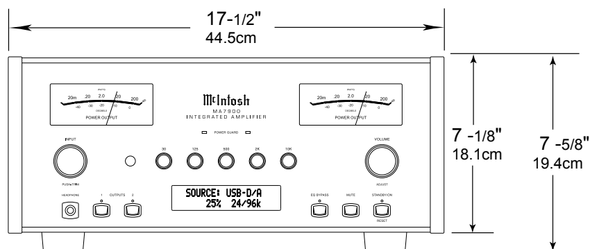
Front View of the MA7900
