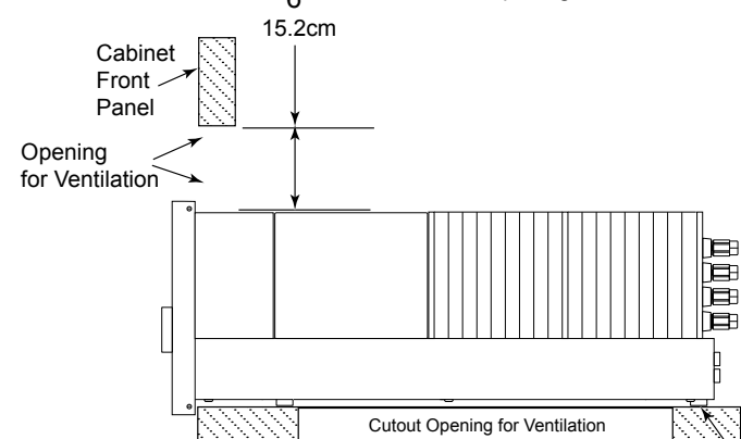
MA7900 Side View in Custom Cabinet
