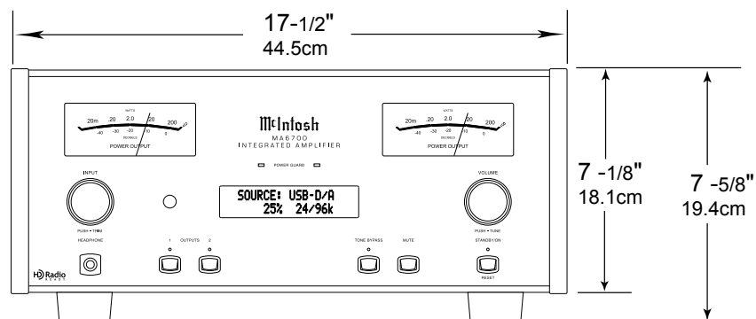
Front View of the MA/MAC6700
