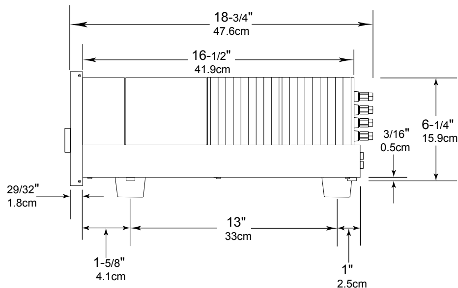
Side View of the MA/MAC6700
