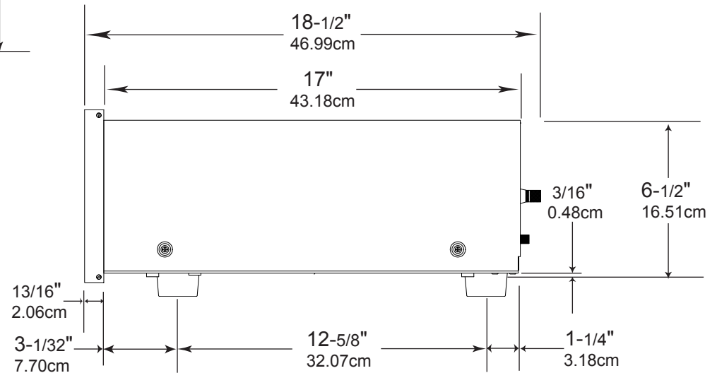
Side View of the MA6300
