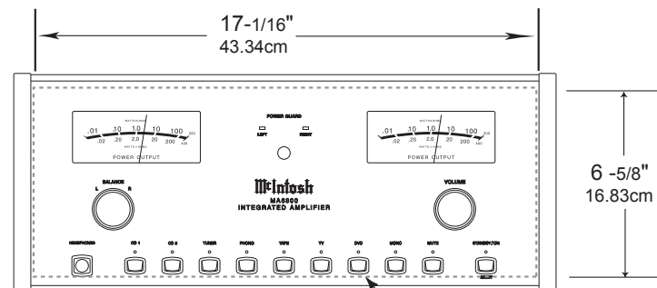
MA6300 Front Panel Custom Cabinet Cutout
