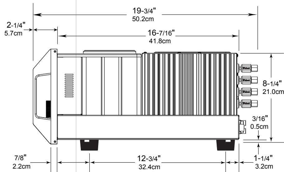
Side View of the MA12000
