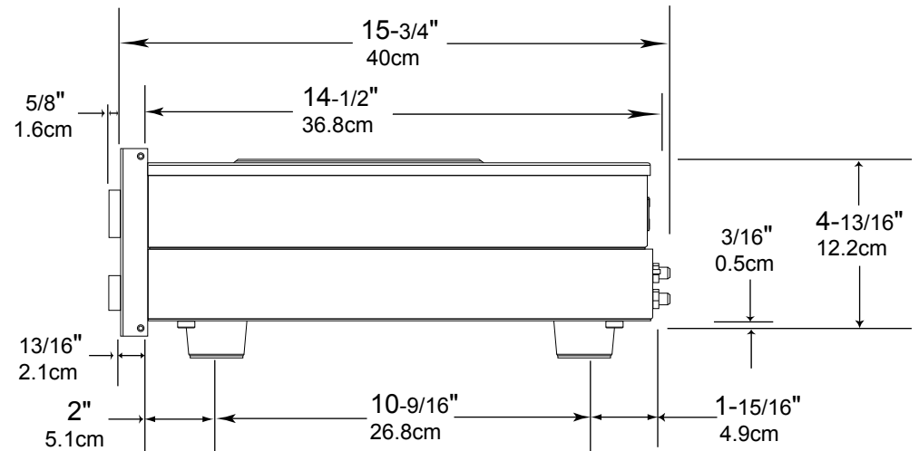
Side View of the C70
