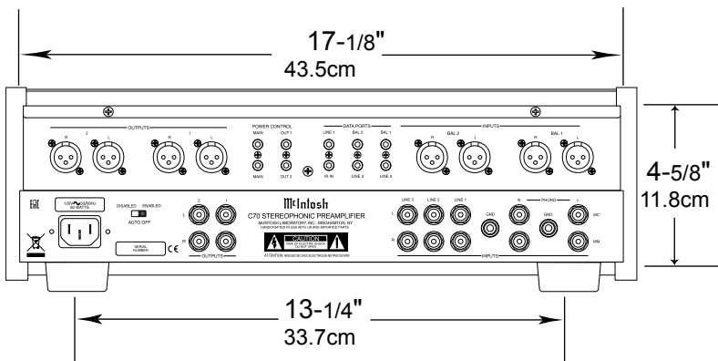
Rear View of the C70
