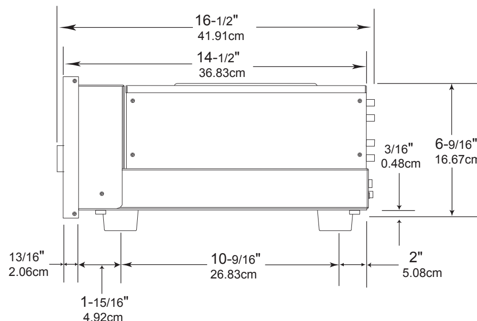
Side View of the C50
