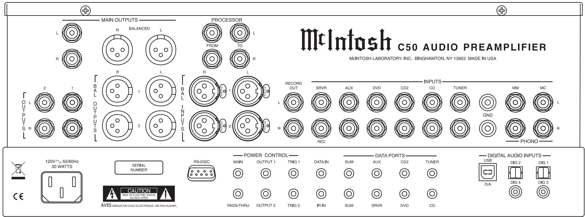
C50 Audio Preamplifier Rear Panel
