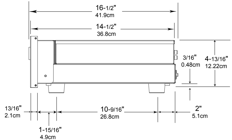
Side View of the C47
