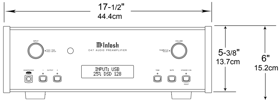
Front View of the C47
