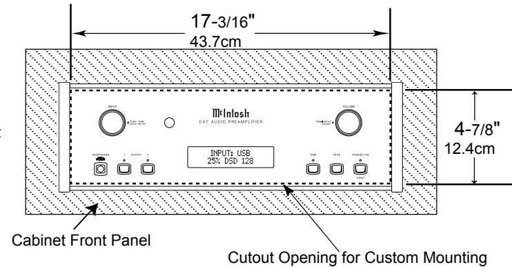
C47 Front Panel Custom Cabinet Cutout
