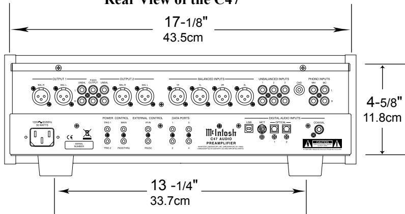
Rear View of the C47
