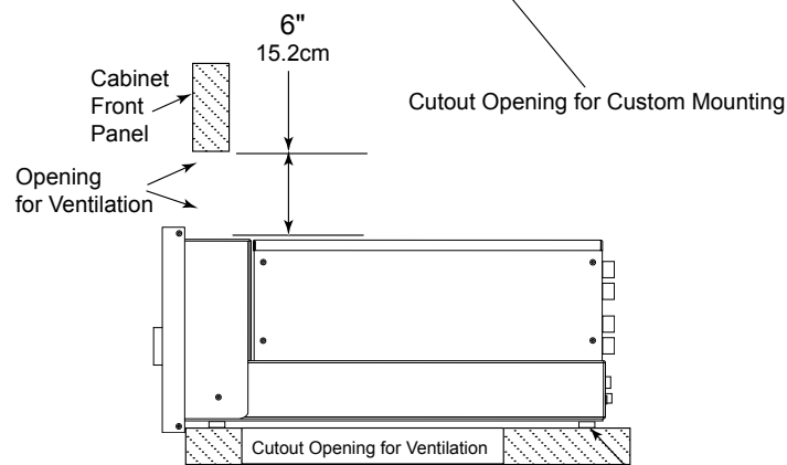
C2700 Side View in Custom Cabinet
