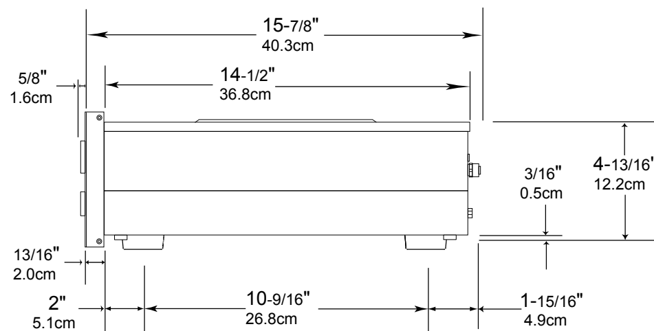
Side View of the C1100C
