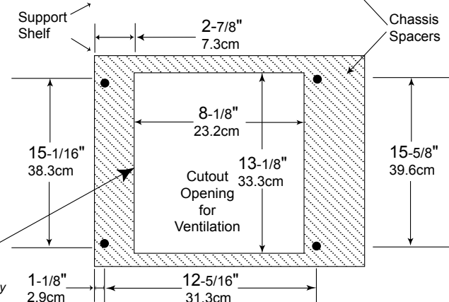
C1100T Bottom View in Custom Cabinet
