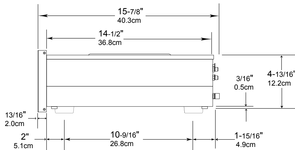
Side View of the C1100T
