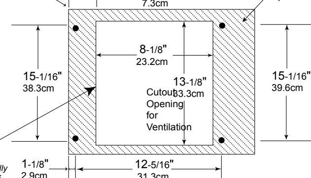
C1100C Bottom View in Custom Cabinet
