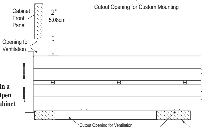
C1000C C1000P C1000T Front Panel Custom Cabinet Cutout
