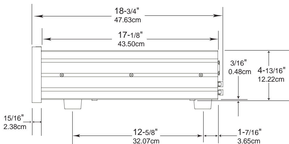
Side View of the C1000T
