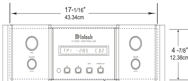
C1000C C1000P C1000T Front Panel Custom Cabinet Cutout
