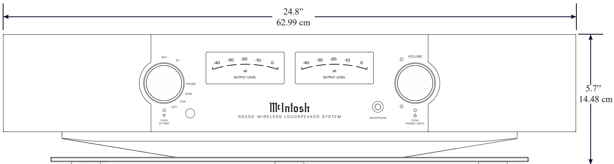
Figure 6– Front View
