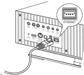
Figure 2– Ethernet connection
