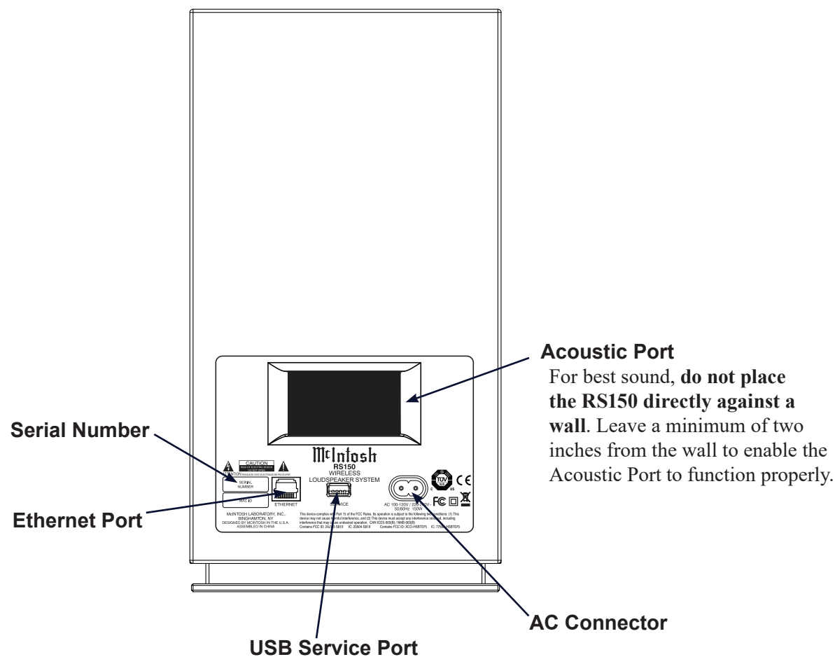
Figure 6– Rear View
