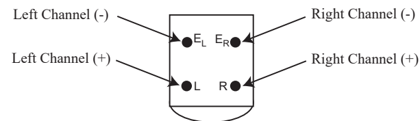
Rear View of Sumiko Amethyst Cartridge
