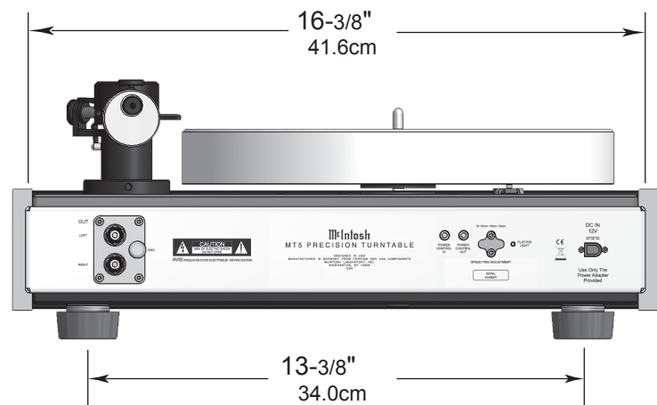
Rear View of the MT5
