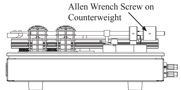
Figure 06- Counterweight Adjustment
