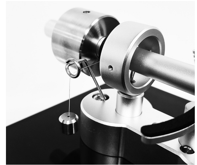
Figure 11– Anti-Skate cable.
