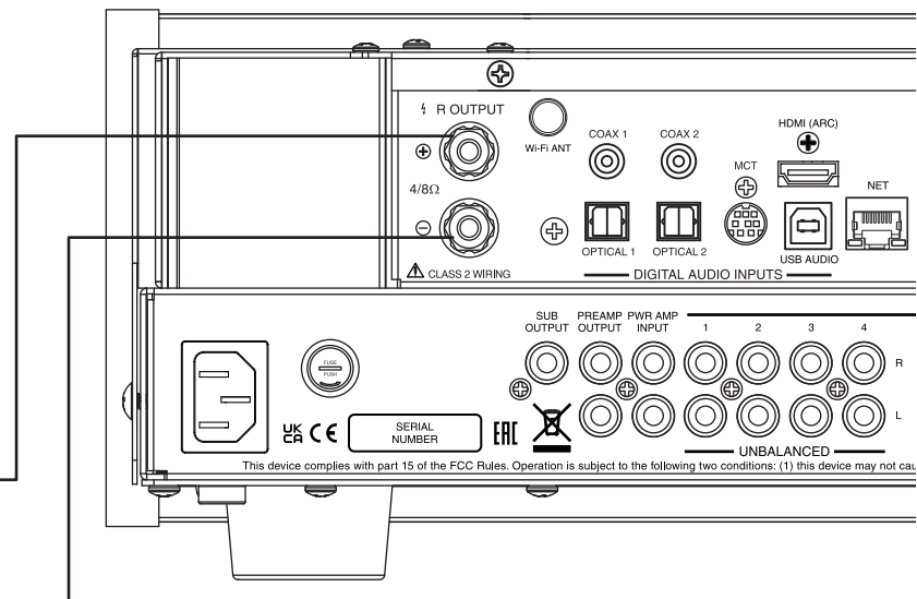
MSA5500 Rear
