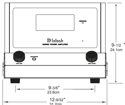
Front View of the MC830
