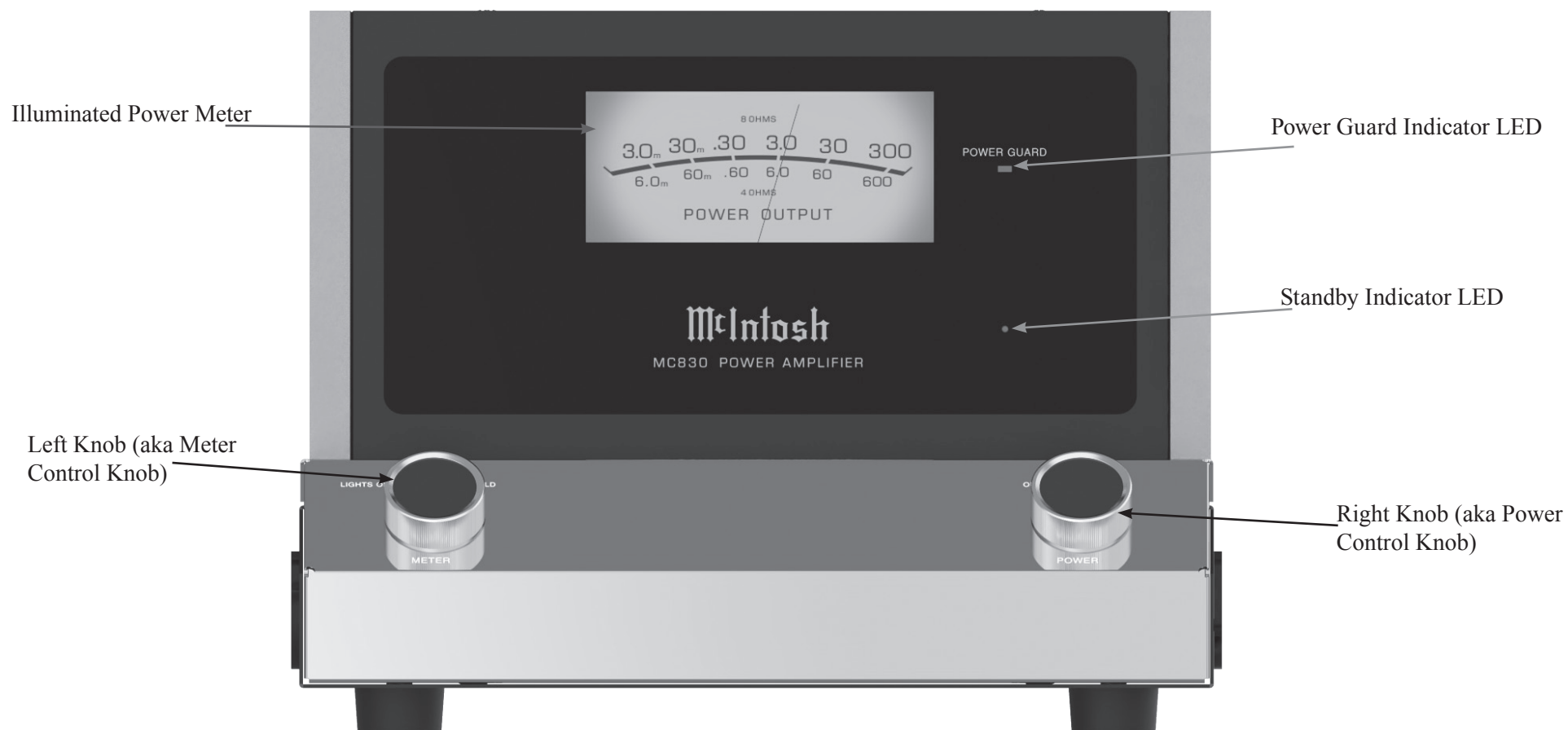
Figure 11– Front Panel
