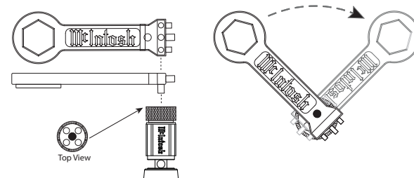
Figure 09– Tightening Binding Post
