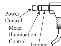
Figure 10– Mini plug for Power Control (Trigger)
