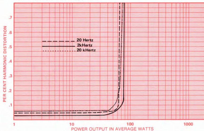
Harmonic Distortion versus Power
