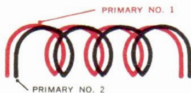
Figure 1. Representation of bifilar winding
