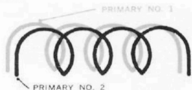
Fig. 1 —Representation of bifilar winding.
