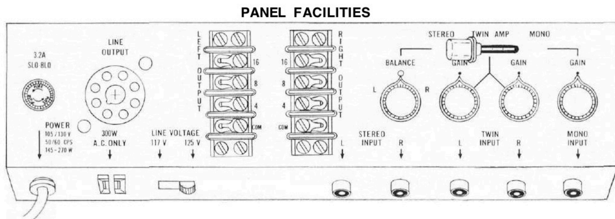
Fig. 3— The end panel of the MC240 showing all input and output facilities.
