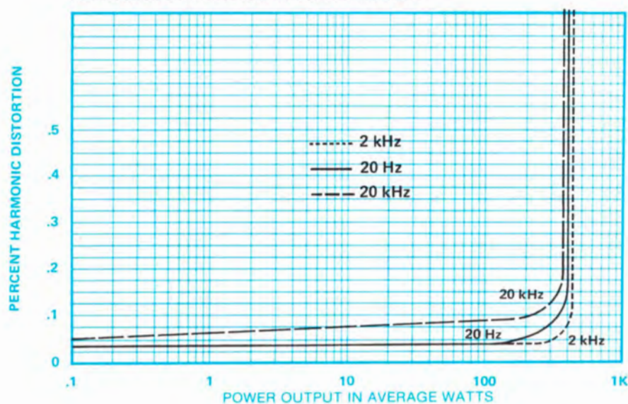
POWER BANDWIDTH
