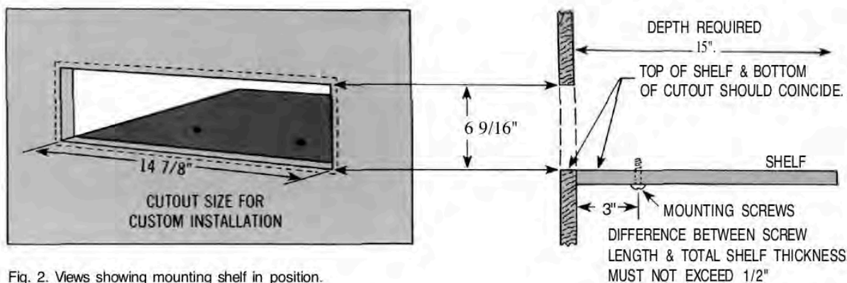
Fig. 2. Views showing mounting shelf in position.
