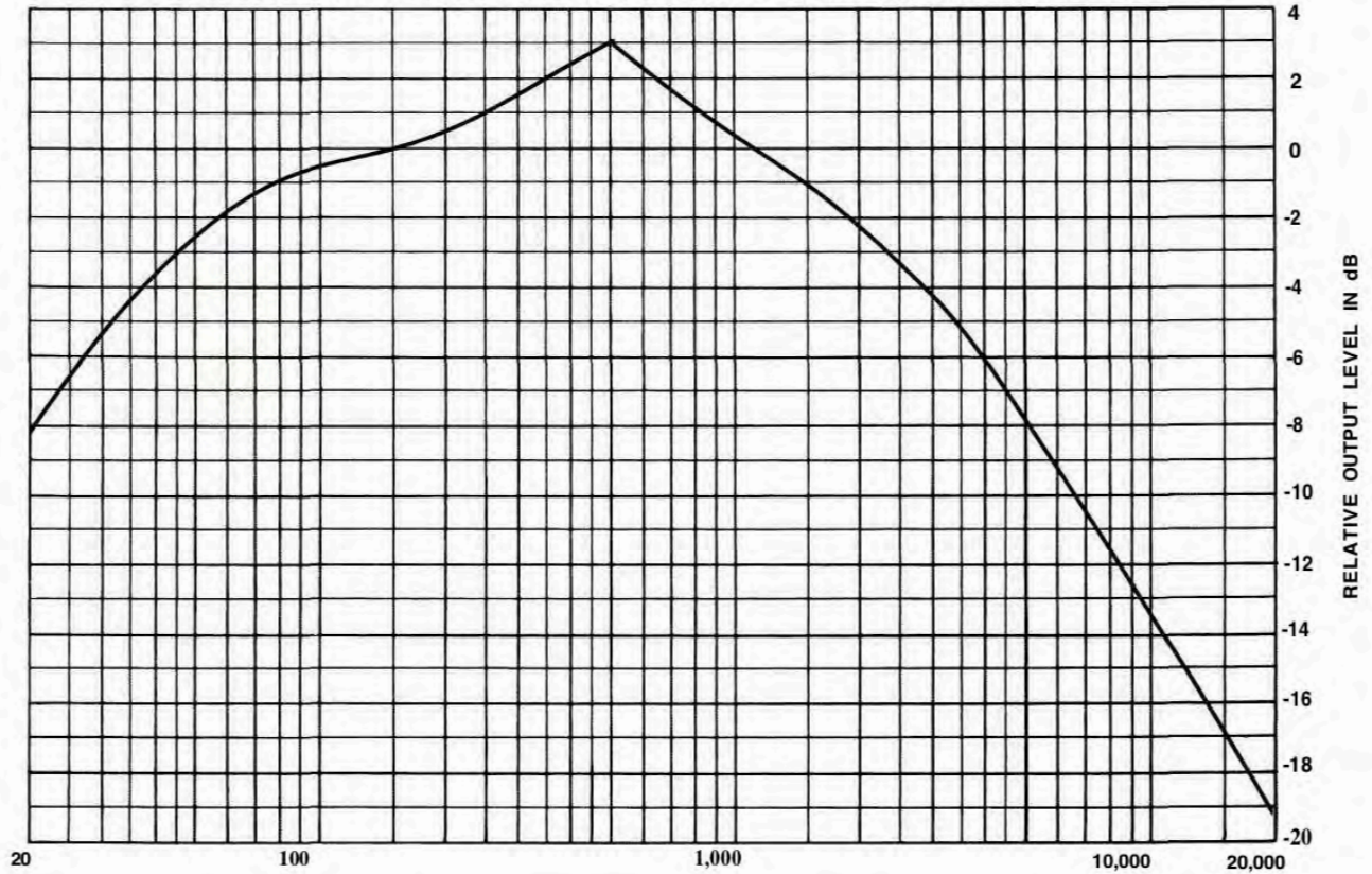
IDEAL RIAA SYSTEM RESPONSE USING CBS STR 100 TEST RECORD
