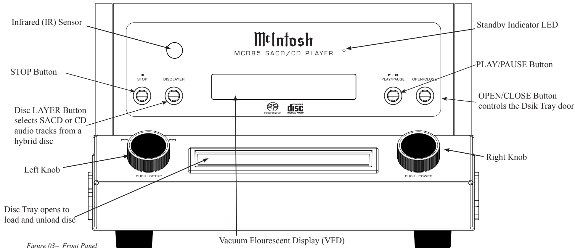
Figure 03– Front Panel
