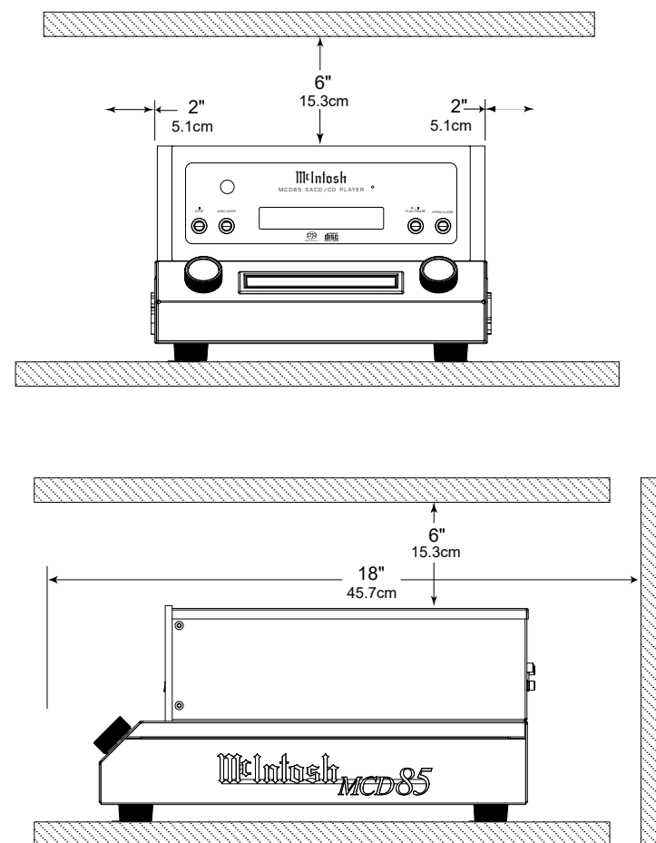
Figure 02– Ventilation requirements
