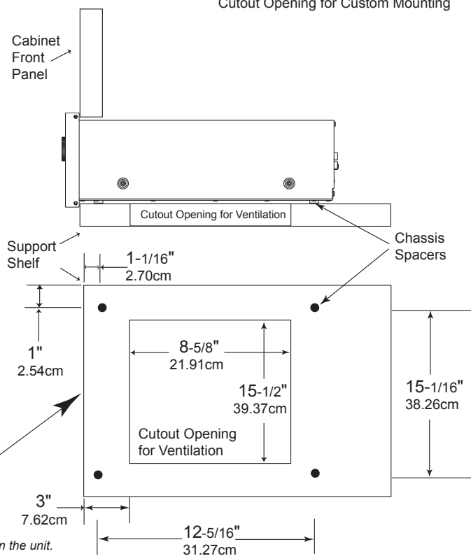
MCD201 Bottom View in Custom Cabinet
