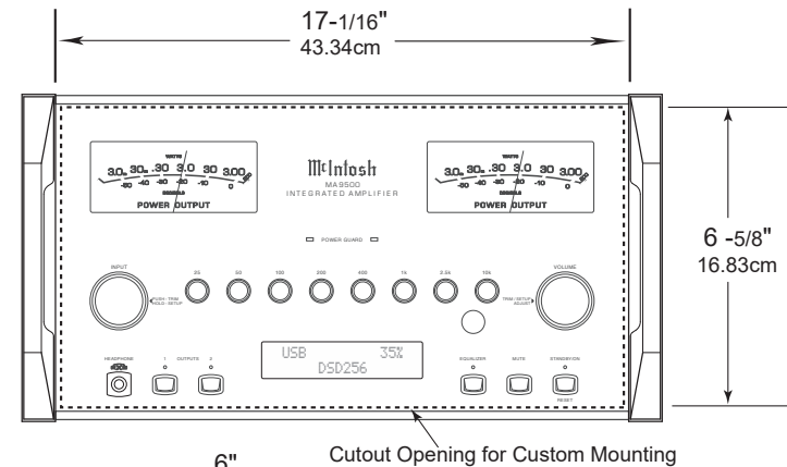
MA9500 Front Panel Custom Cabinet Cutout
