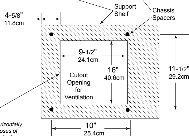
MA9000 Bottom View in Custom Cabinet
