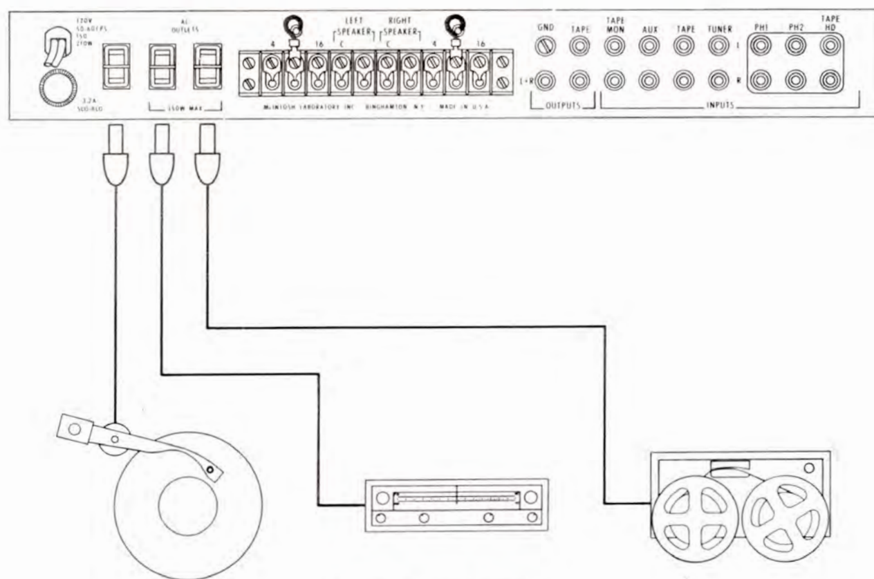
Figure 23. AC CONNECTIONS
