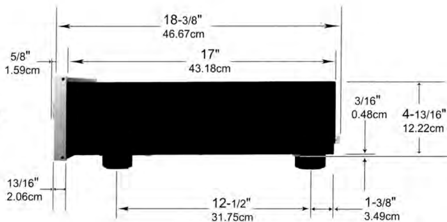
Side View of the C200C
