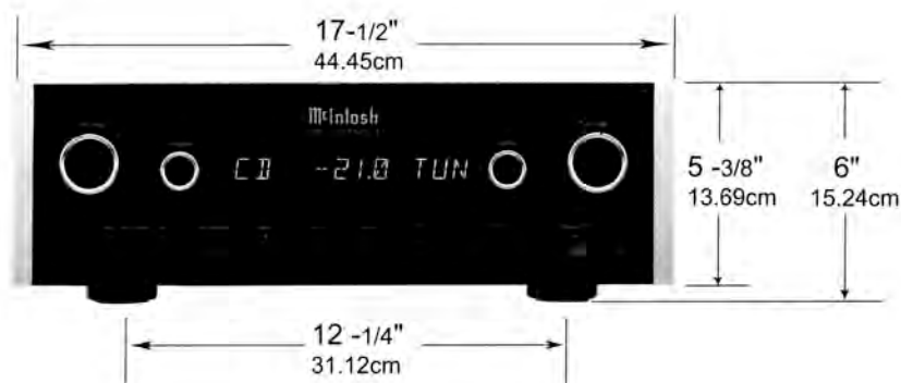
Front View of the C200C
