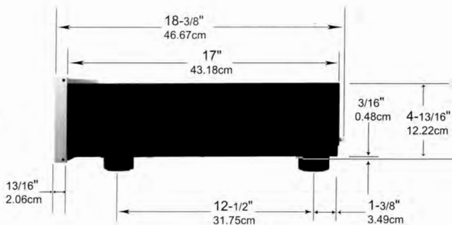
Side View of the C200P
