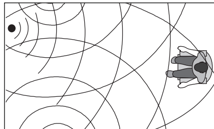
Figure 6-7. As can be seen here, point source concepts invite a great deal of room interaction. While delivering good frequency response to a large listening audience, imaging is consequently confused and blurred.
