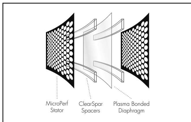
Figure 13. Cut away view of an XStat™ electrostatic transducer. Notice the simplicity due to minimal parts usage.
