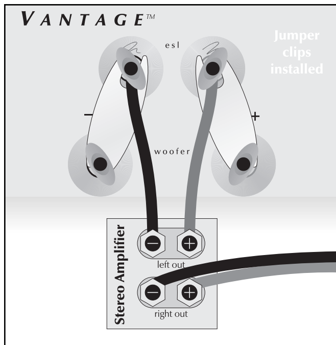
Figure 2. Single-wire connection. One channel shown.
