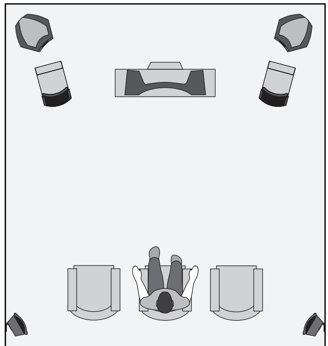
Figure 12. Vantage speakers as front channels, the Stage as the center channel, Script i speakers as side surround (effects) channels, and Descent subwoofers as 0.1 (effects) channel.
