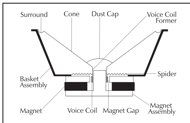
Figure 14. Cut away view of a typical moving coil driver. Notice the complexity due to the high number of parts.
