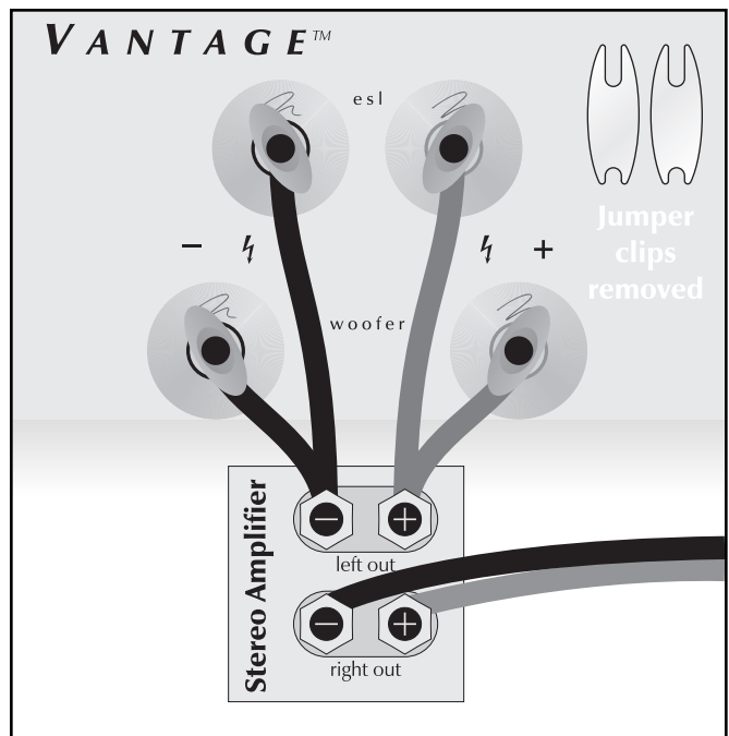
Figure 3. Bi-wire connection. One channel shown.
