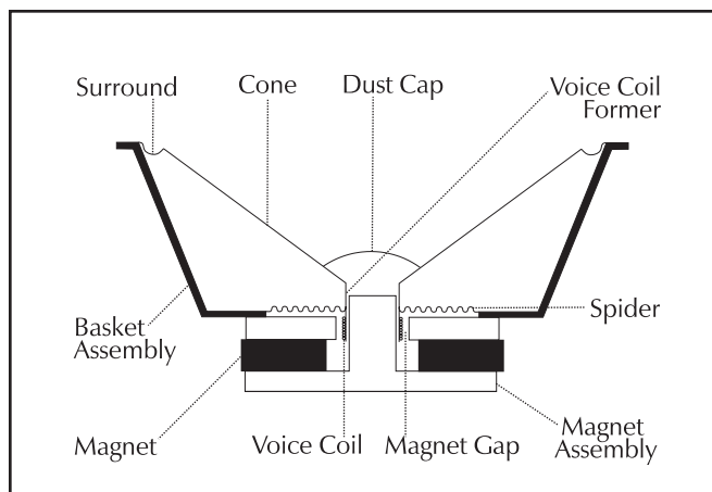
Figure 16. Cut away view of a typical moving coil driver. Notice the complexity due to the high number of parts.
