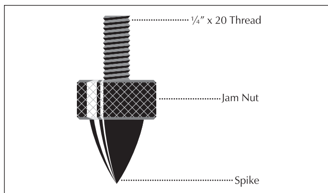
Figure 7. The ETC Spike.
