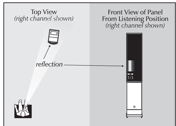
Figure 3. Flashlight toe-in technique.
