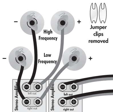
Fig. 4: Vertical bi-amplification connection. One channel shown.
