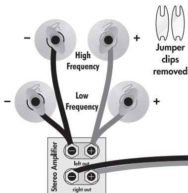
Fig. 2: Bi-wire connection. One channel shown.
