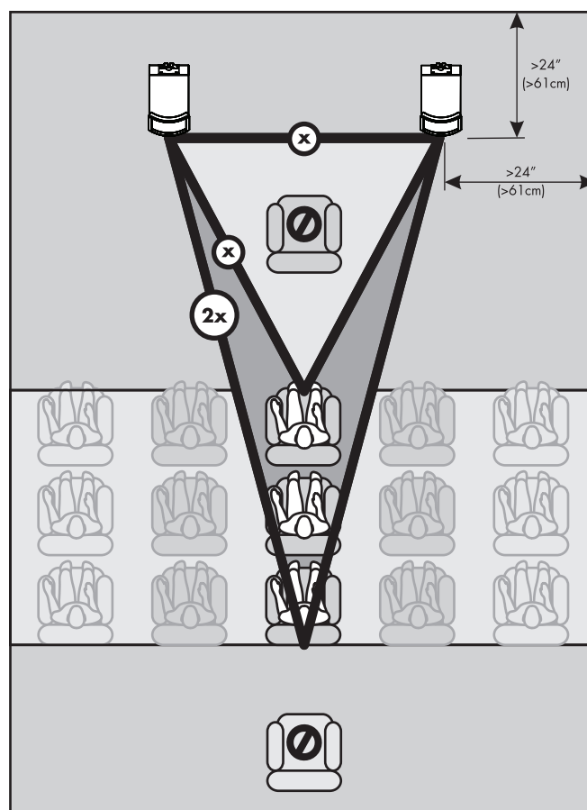
Figure 2: Final placement. Measure the distance from the front wall to the center of the speakers (inches) and multiply the figure by 0.618
