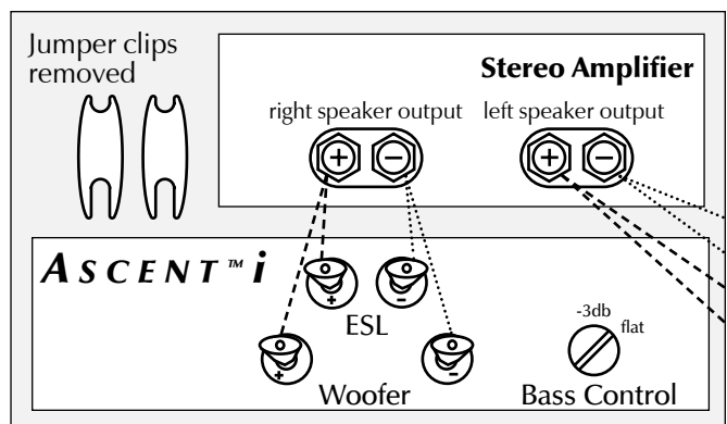
Figure 3. Bi-wire connection. One channel shown.
