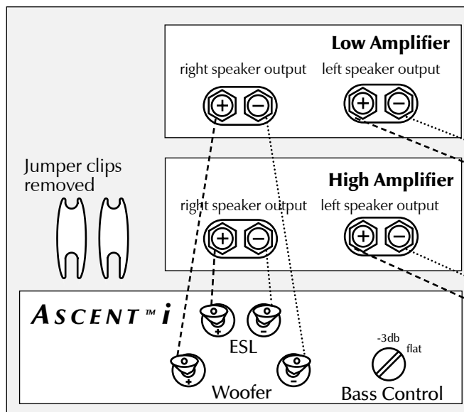
Figure 4. Horizontal passive bi-amplification. One channel shown.
