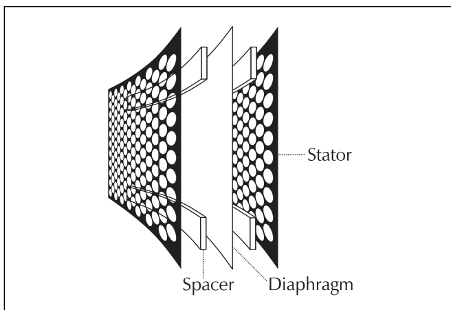
Figure 18. Cut-away view of an electrostatic transducer. Notice the simplicity due to minimal parts usage.
