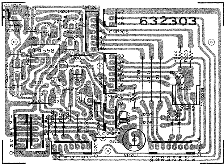
MAIN CONTROL P.W.B. (2)
