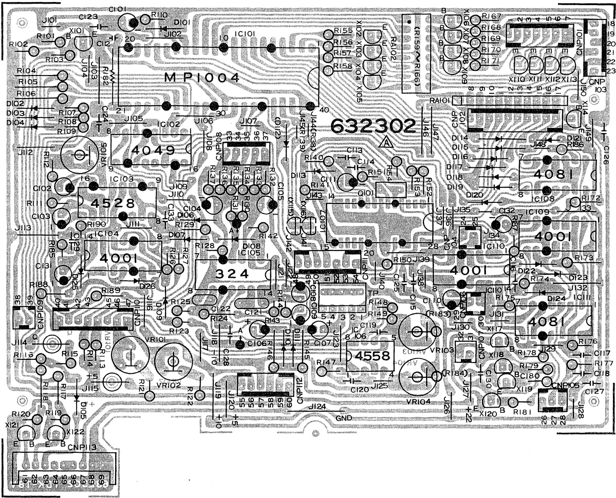
MAIN CONTROL P.W.B. (1)
