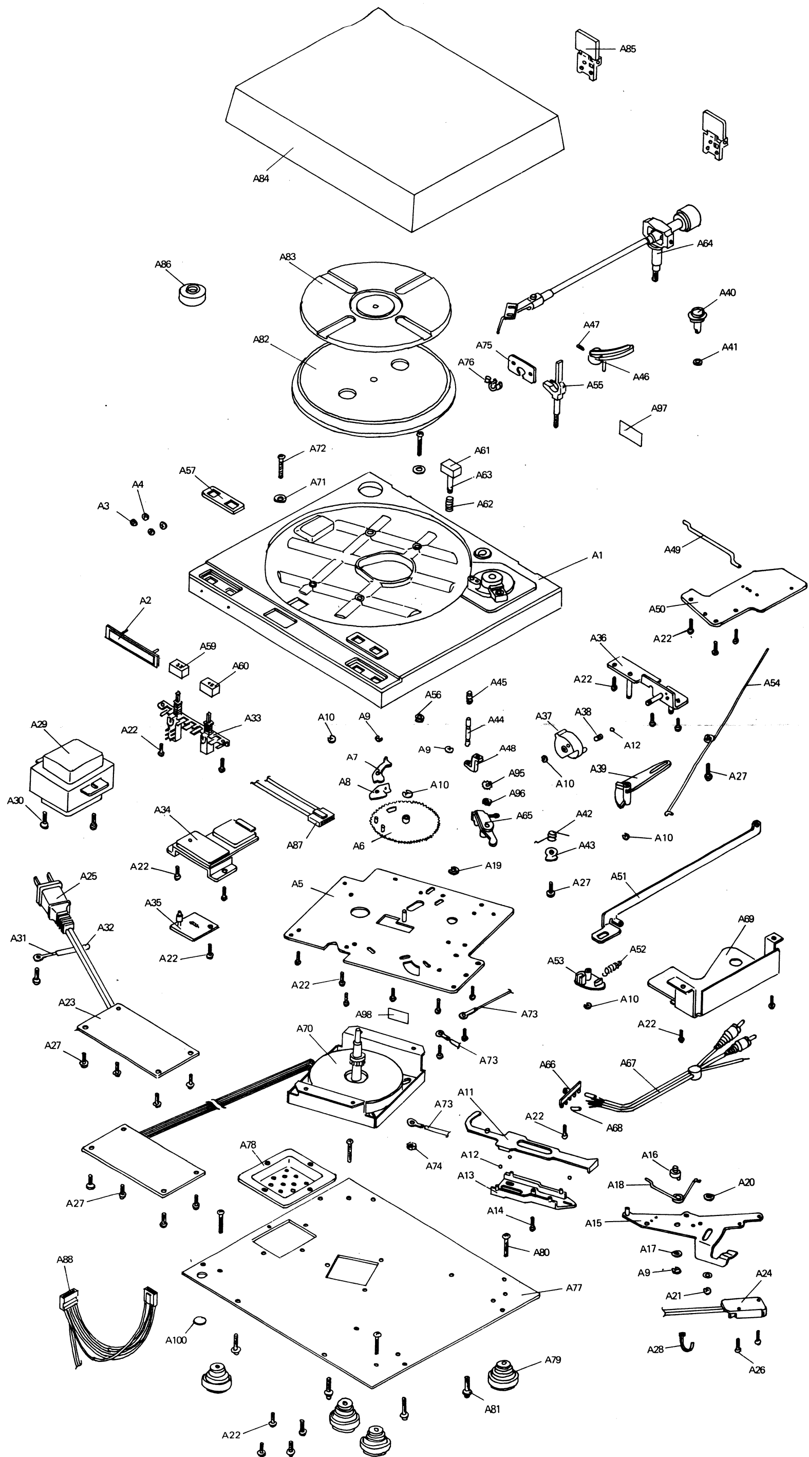
MAIN CHASSIS ASSEMBLY
