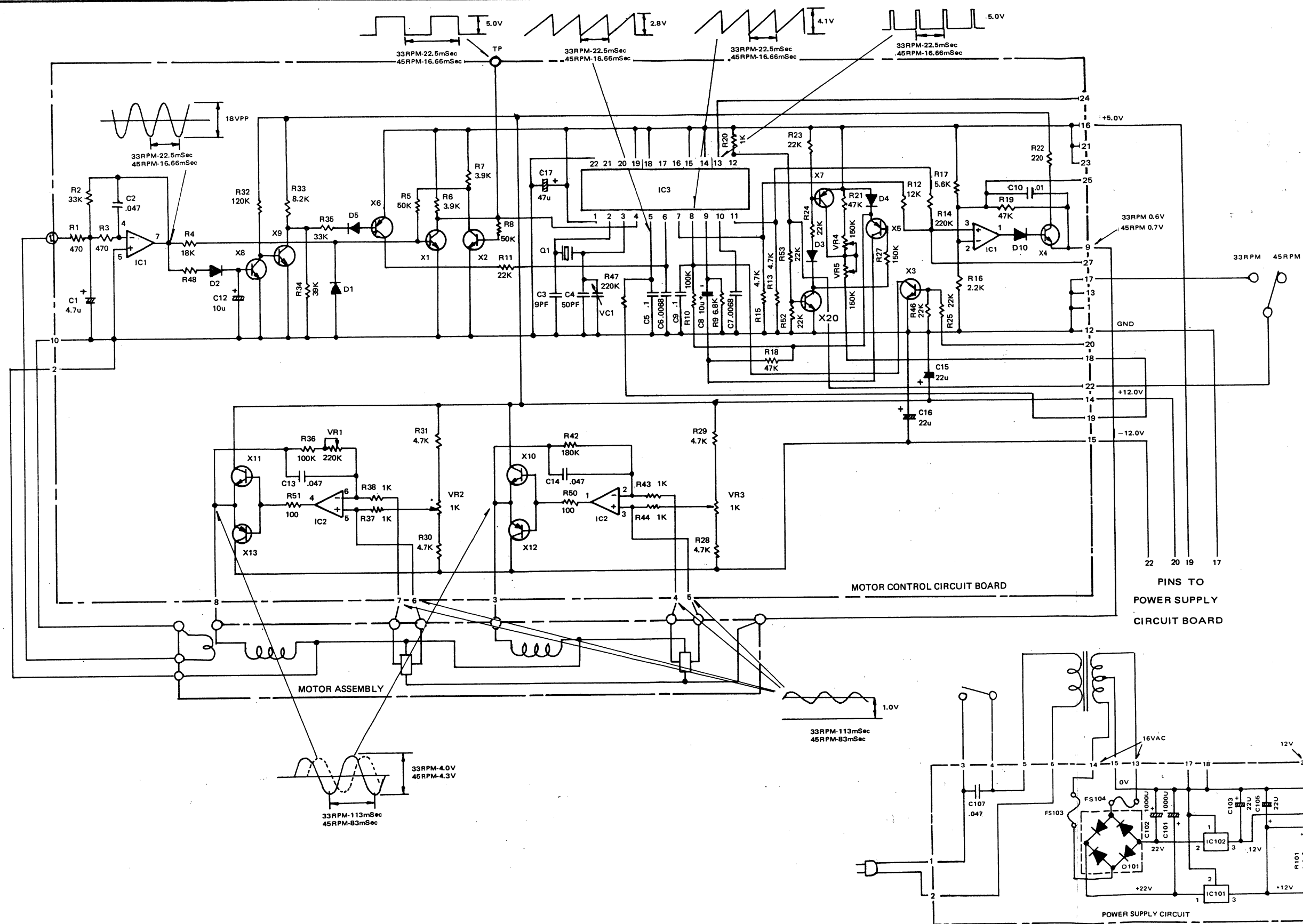
ELECTRICAL SCHEMATIC TT-4000
