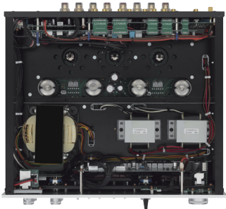
Internal configuration
